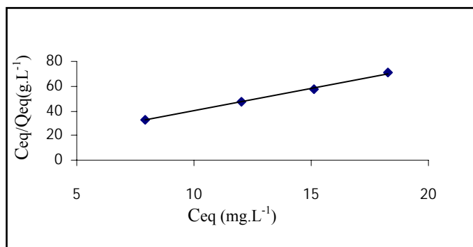
Fig.23. Langmuir isotherm of TBO with MnO 2 /TiO 2 .
