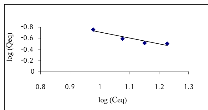
Fig.10. Freundlich isotherm of TBO at pH=12.
